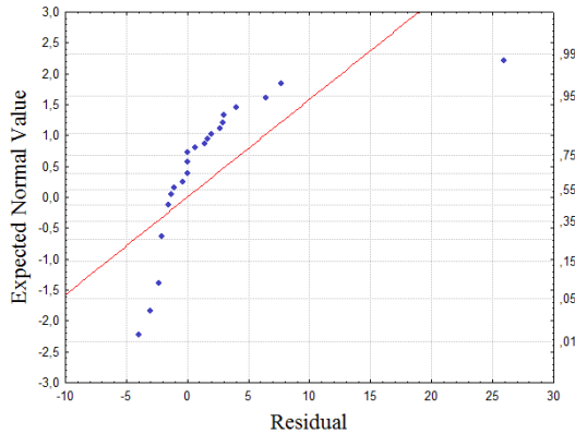
Figure 3: Normal probability plot of raw residuals
