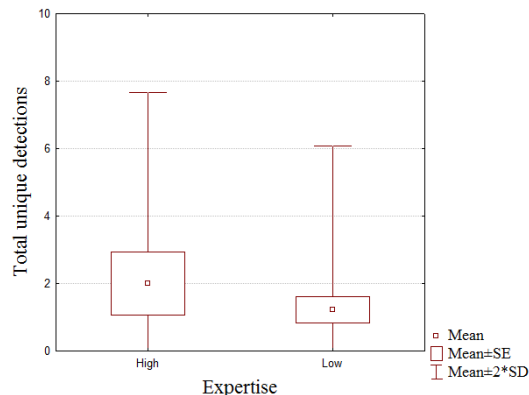
Figure 8: Box plot of unique detections by computer expertise
