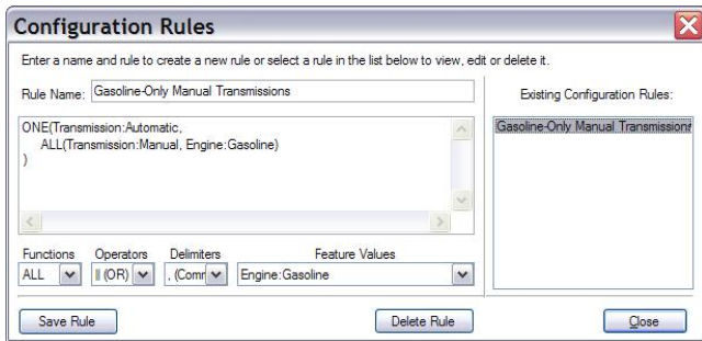
Figure 3. An example configuration rule shown in CASE-FX
