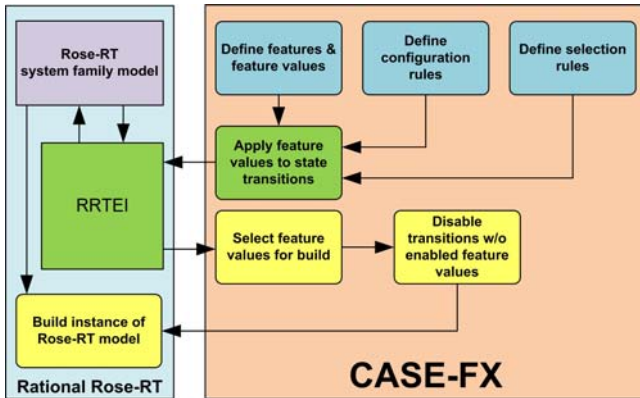
Figure 2. Flow diagram of CASE-FX working with Rose-RT
