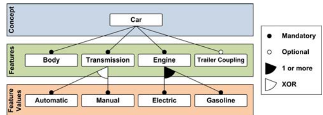
Figure 1. An example feature diagram of a Car [4]
