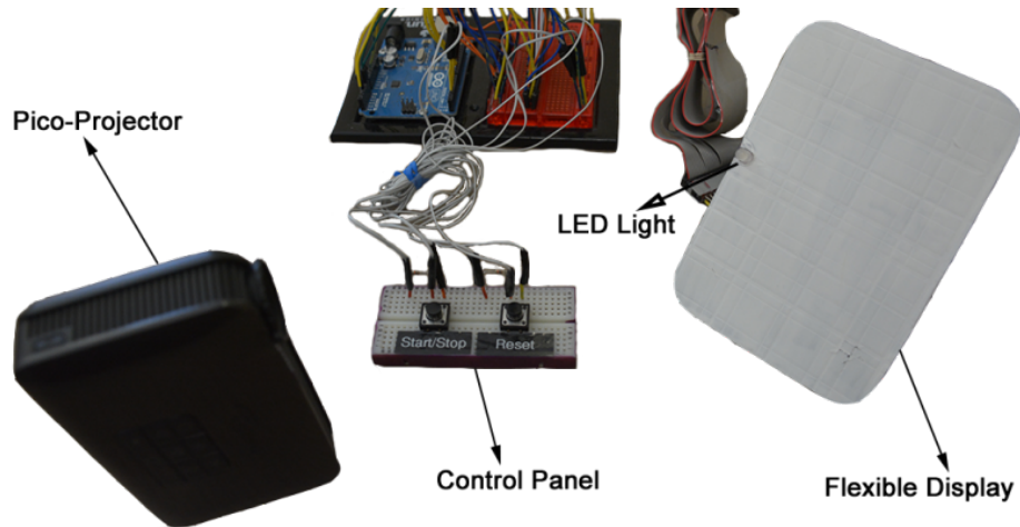
Fig. 1 Hardware components of the flexible display prototype
