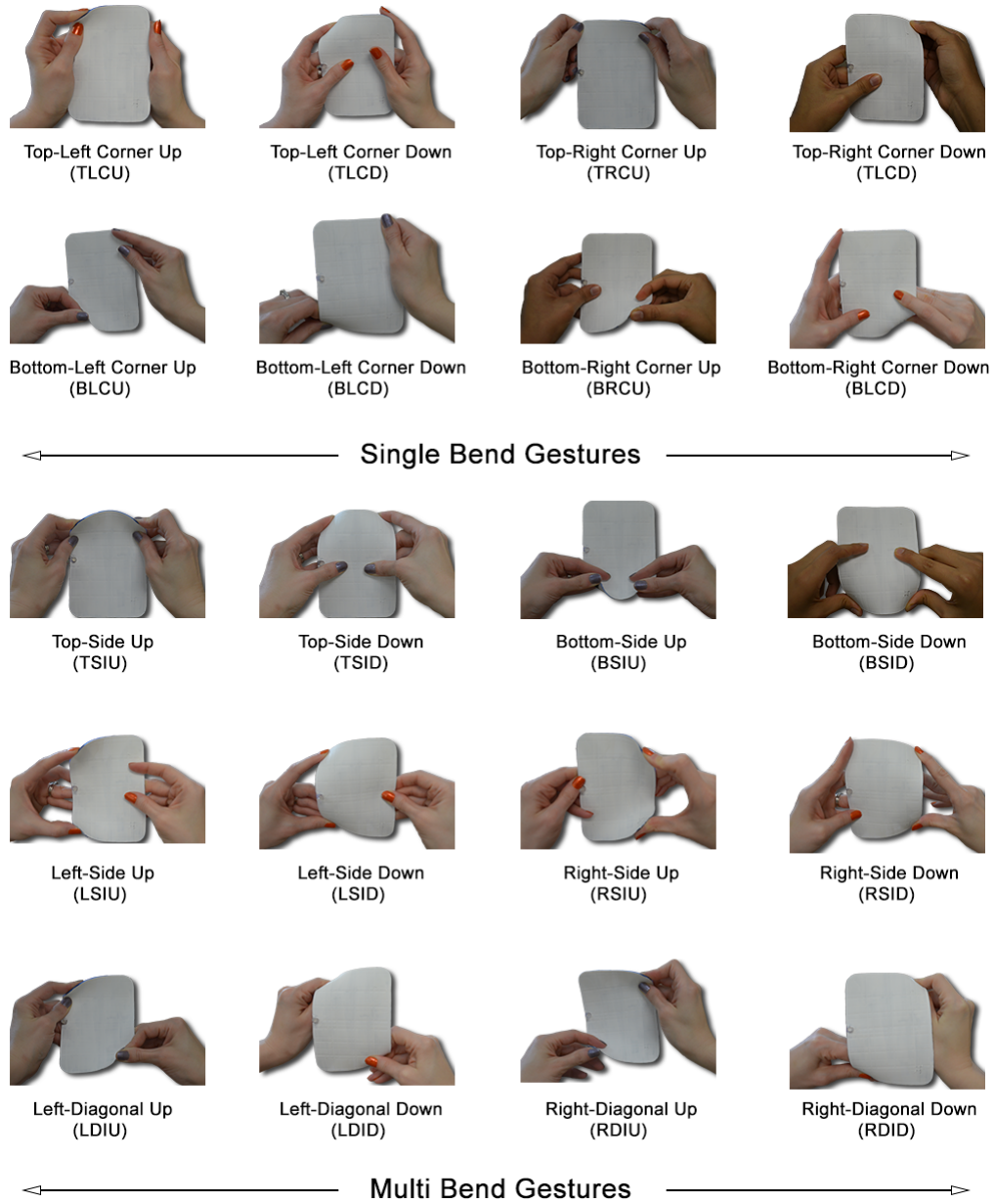
Fig. 12 The set of bend gestures available on the flexible display prototype
