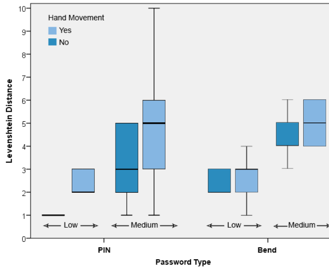
Fig. 10 Levenshtein distance for PINs and Bend Passwords. Low and medium are the theoretical passwords strengths
